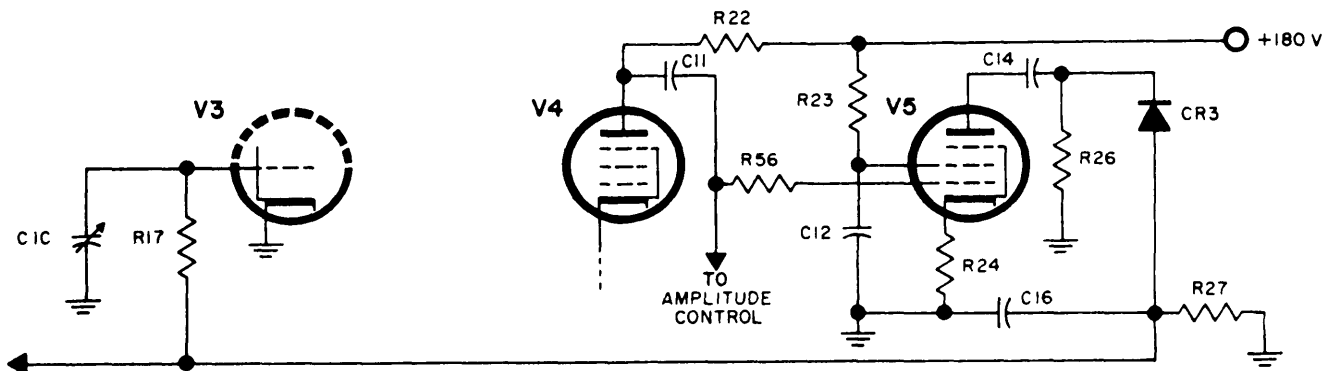
Figure 3-3. Simplified Diagram of High Frequency Oscillator AVC System
